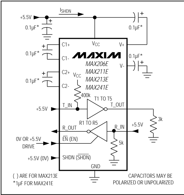
Figure 1. Shutdown-Current Test Circuit (MAX206E, MAX211E/MAX213E/MAX241E)
