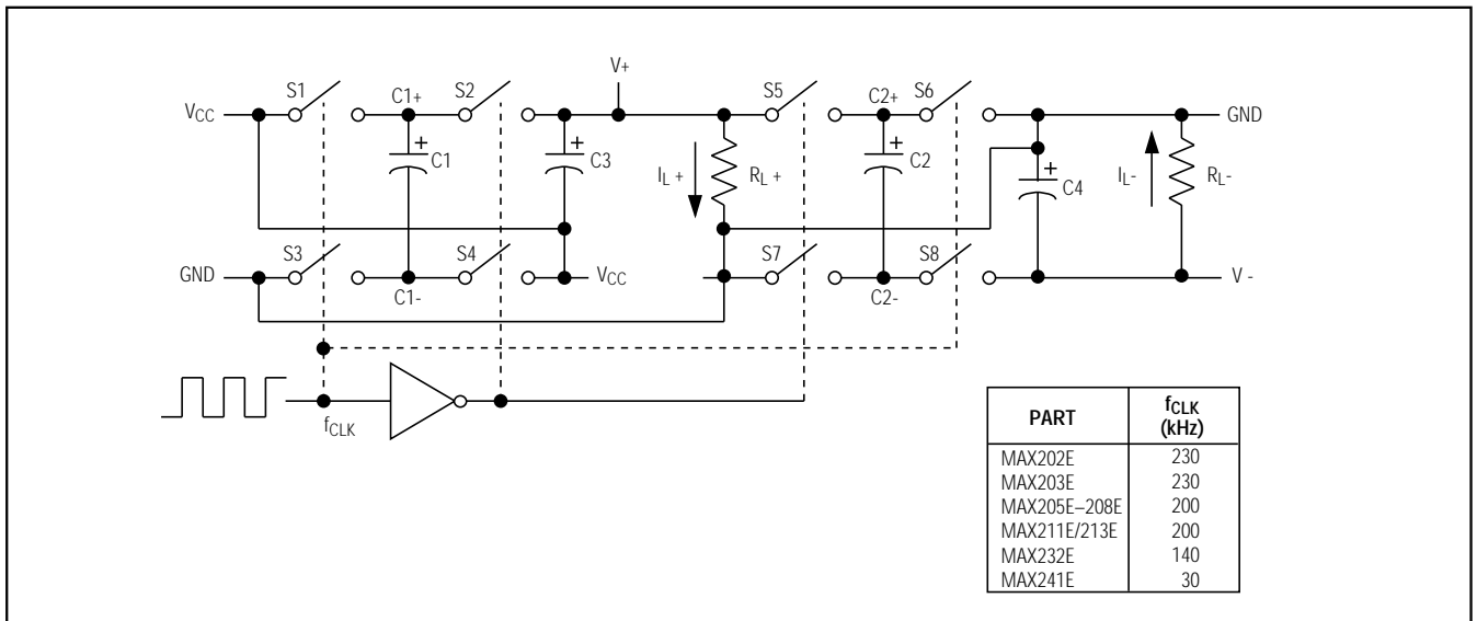
Figure 4. Charge-Pump Diagram
