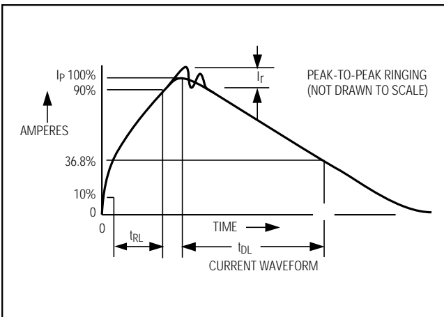
Figure 6b. Human Body Model Current Waveform
